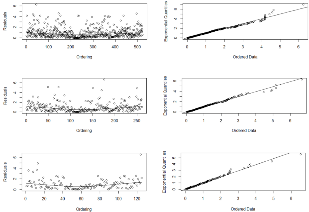
Figure 4. Residual plots (left) and Q-Q plots (right) for the fitting of GEVD to Dow Jones US Mining Index, with block sizes 5 (row 1), 10 (row 2) and 21 (row 3)
