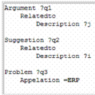
Figure 10: The Request In The Conceptual Graph Formalism
